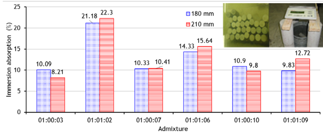
Figure 11 - Immersion absorption
