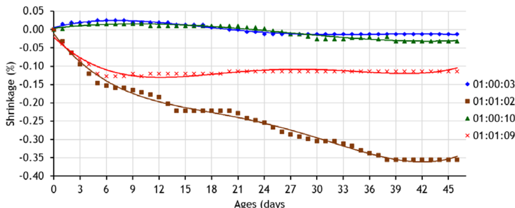
Figure 12 - Shrinkage for the workability - 180 mm
