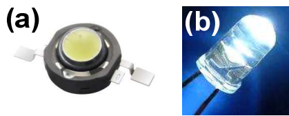
Figura 34 – Dois tipos de LED (a) LED HP e (b) LED HB.
