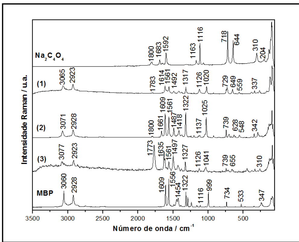
Figura 24 Espectros Raman dos compostos [\text{Co}(\text{MBP})_2(\text{C}_4\text{O}_4)] ( 1 ), [\text{Ni}(\text{MBP})_3](\text{C}_4\text{O}_4) \cdot 3\text{H}_2\text{O} ( 2 ) e \{[\text{Cu}_2(\text{MBP})_2(\text{C}_4\text{O}_4)_2(\text{H}_2\text{O})_4]\}_n ( 3 ) bem como para os ligantes MBP e \text{Na}_2\text{C}_4\text{O}_4 .
