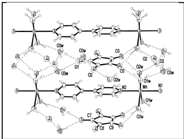
Figura 89 Polímero [\{\text{Mn}(4,4'\text{-bipy})(\text{H}_2\text{O})_4\}(\text{C}_5\text{O}_5)(\text{H}_2\text{O})_2]_n , descrito na literatura.
