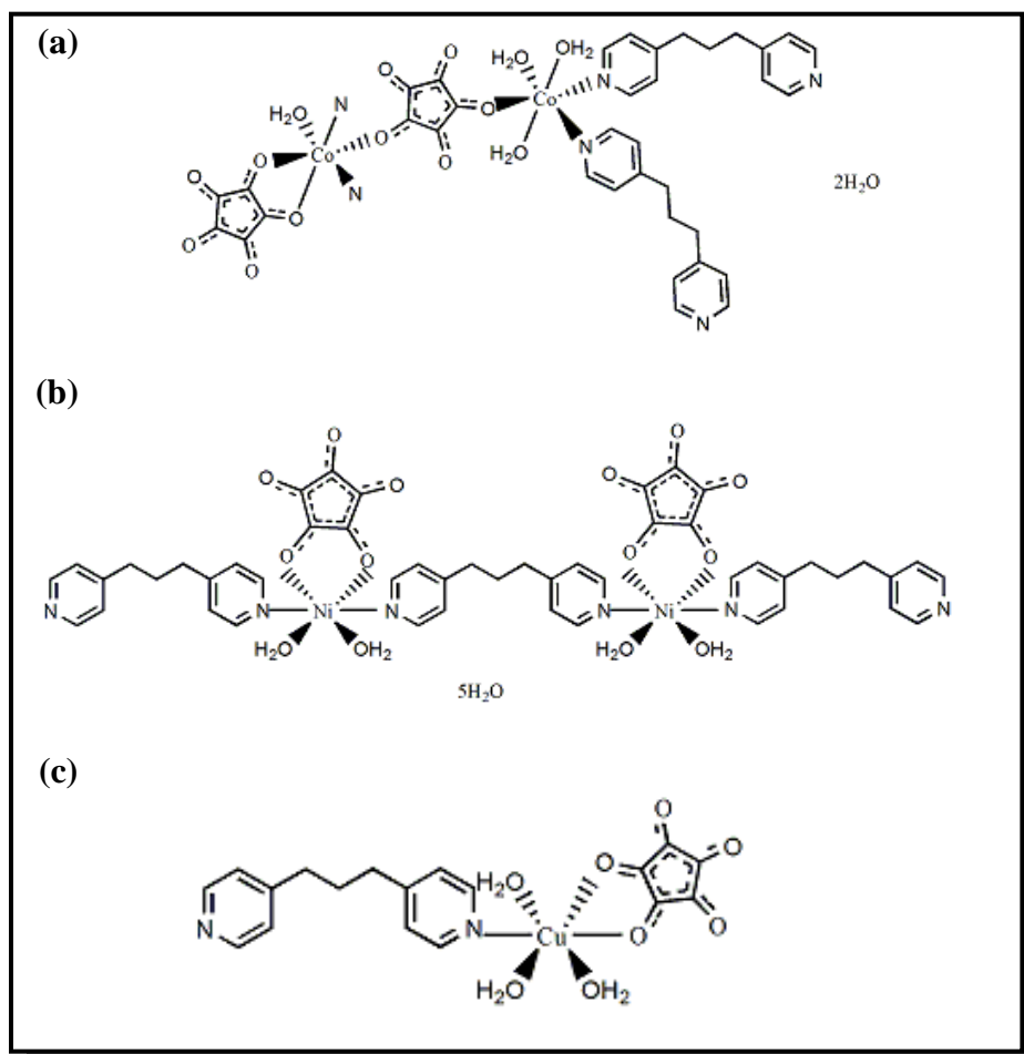
Figura 65 Representação das propostas estruturais para os compostos: (a) \{[\text{Co}_2(\text{BPP})_2(\text{C}_5\text{O}_5)_2(\text{H}_2\text{O})_4] \cdot 2\text{H}_2\text{O}\}_n ( 11 ), (b) \{[\text{Ni}_2(\text{BPP})_3(\text{C}_5\text{O}_5)_2(\text{H}_2\text{O})_4] \cdot 5\text{H}_2\text{O}\}_n ( 12 ) e (c) \{[\text{Cu}(\text{BPP})(\text{C}_5\text{O}_5)(\text{H}_2\text{O})_3]\}_n ( 13 ).
