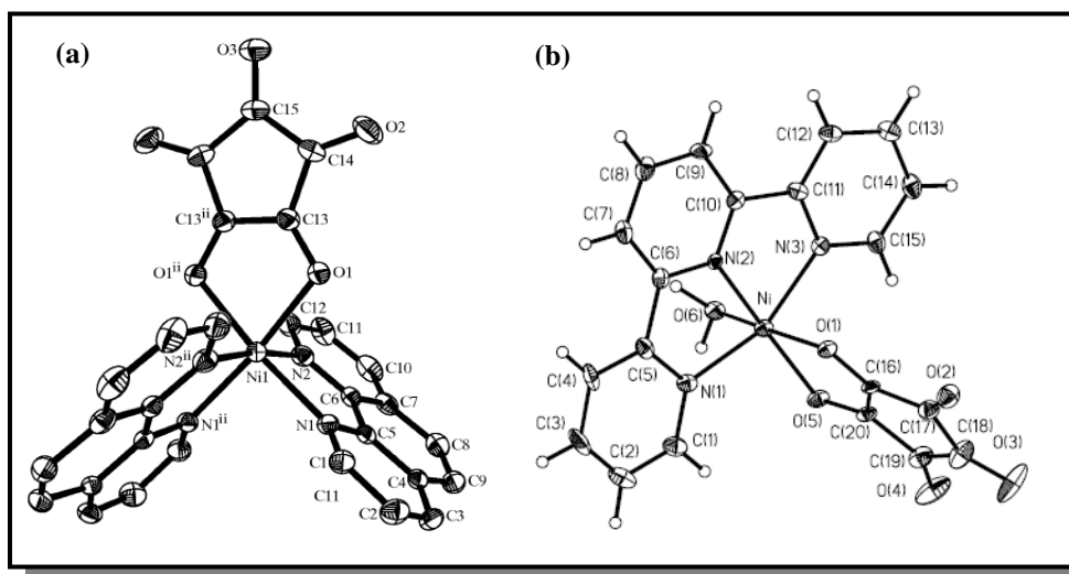
Figura 60 Estruturas propostas na literatura para os compostos: (a) [\text{Ni}(\text{C}_{12}\text{H}_8\text{N}_2)_2(\text{C}_5\text{O}_5)] e (b) [\text{Ni}(\text{terpy})(\text{C}_5\text{O}_5)(\text{H}_2\text{O})] \cdot \text{H}_2\text{O} .
