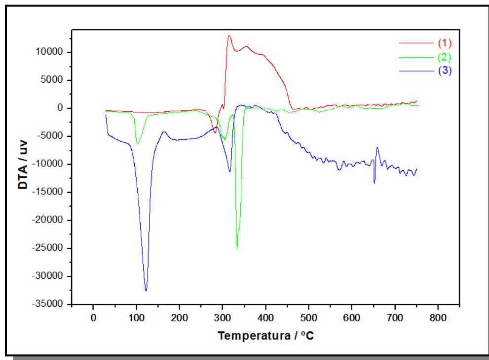
Figura 22 Curvas DTA para os compostos [\text{Co}(\text{MBP})_2(\text{C}_4\text{O}_4)] (1) , [\text{Ni}(\text{MBP})_3](\text{C}_4\text{O}_4) \cdot 3\text{H}_2\text{O} (2) e \{[\text{Cu}_2(\text{MBP})_2(\text{C}_4\text{O}_4)_2(\text{H}_2\text{O})_4]\}_n (3) .
