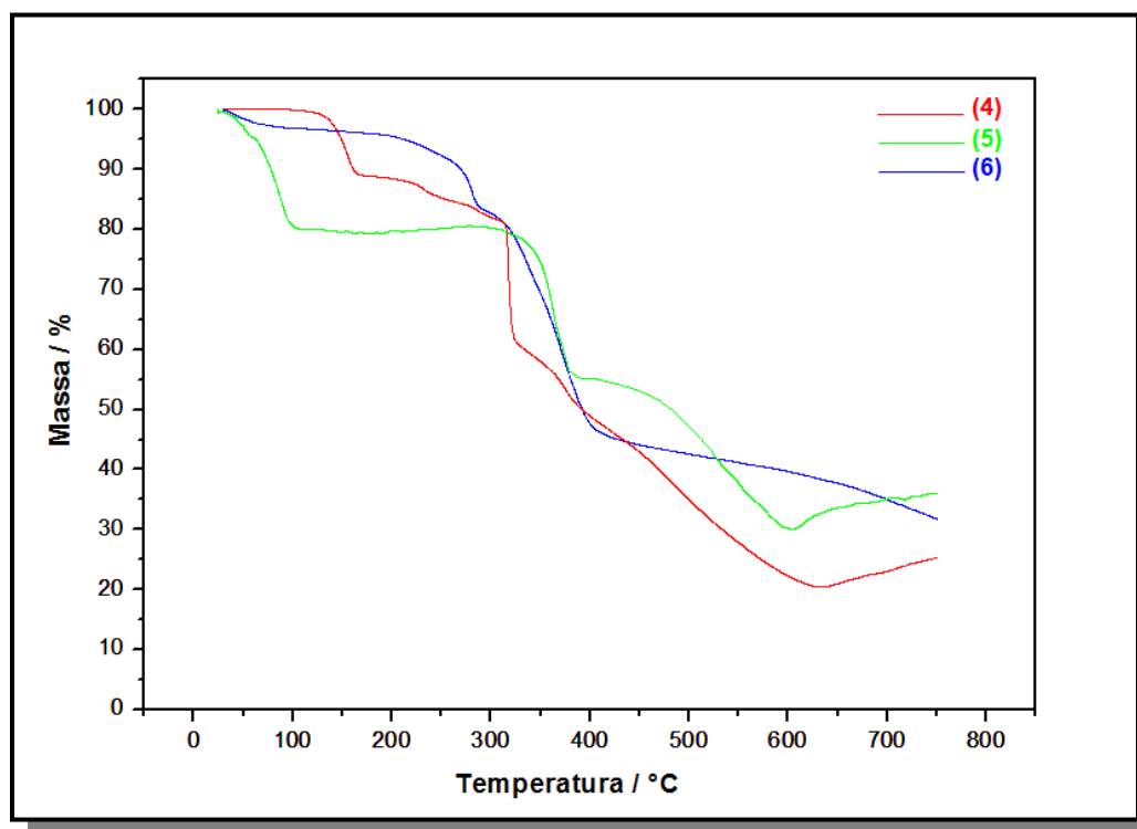
Figura 33 Curvas TG para os compostos [\text{Co}_2(\text{TPP})(\text{C}_4\text{O}_4)_2(\text{H}_2\text{O})_2] \cdot 2\text{H}_2\text{O} ( 4 ), [\text{Ni}_2(\text{TPP})(\text{C}_4\text{O}_4)(\text{H}_2\text{O})_2\text{Cl}_2] \cdot 7\text{H}_2\text{O} ( 5 ) e [\text{Cu}_2(\text{TPP})(\text{H}_2\text{O})_2\text{Cl}_2](\text{C}_4\text{O}_4) \cdot 2\text{H}_2\text{O} ( 6 ).
