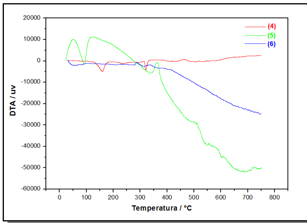
Figura 34 Curva DTA para os compostos [\text{Co}_2(\text{TPP})(\text{C}_4\text{O}_4)_2(\text{H}_2\text{O})_2] \cdot 2\text{H}_2\text{O} (4) , [\text{Ni}_2(\text{TPP})(\text{C}_4\text{O}_4)(\text{H}_2\text{O})_2\text{Cl}_2]7\text{H}_2\text{O} (5) e [\text{Cu}_2(\text{TPP})(\text{H}_2\text{O})_2\text{Cl}_2](\text{C}_4\text{O}_4)2\text{H}_2\text{O} (6) .
