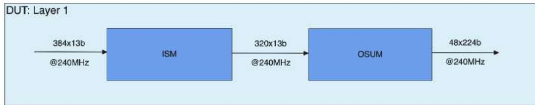
Figure 41 – Simulation strategy for Layer 1: isolated HLS block verification in a single clock domain.
