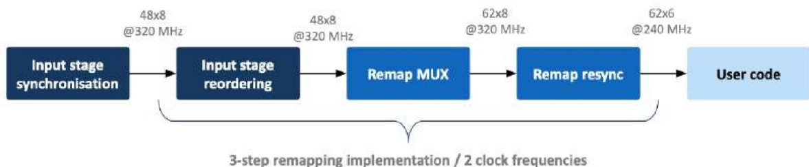
Figure 14 – Three-step remapping implementation in the LATOME v5 firmware.
