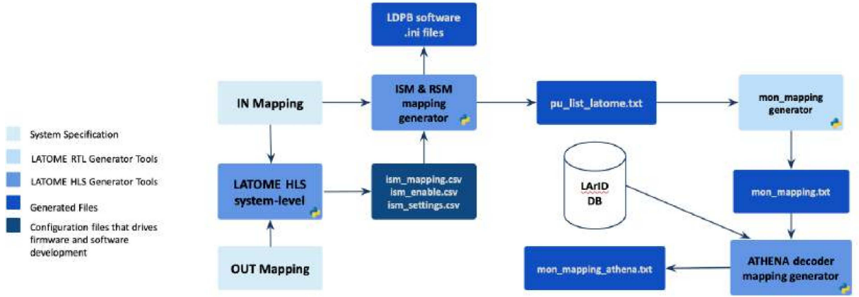
Figure 35 – LATOME HLS software infrastructure
