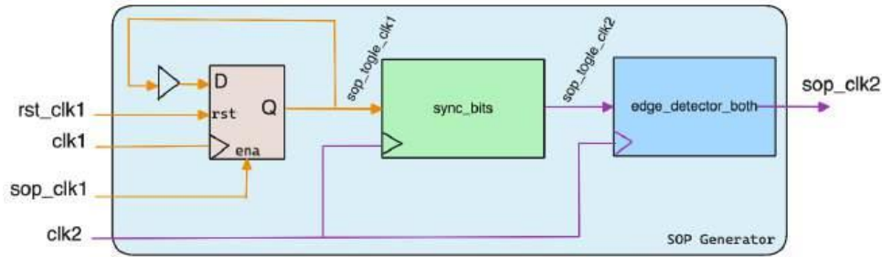
Figure 25 – SOP generator: produces a reference pulse that marks the start of each bunch crossing and distributes it to the S2P converters.
